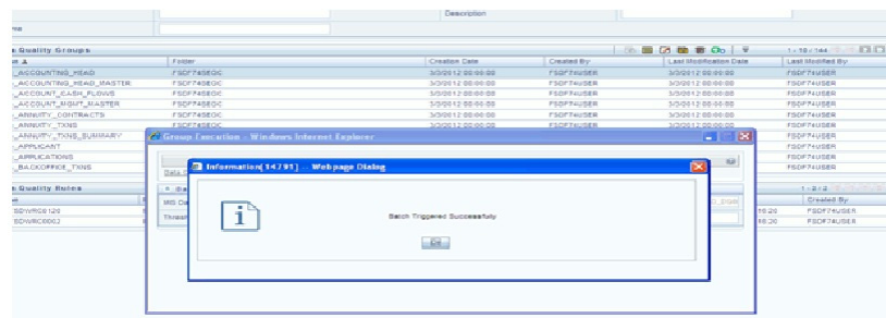
Figure 20. Execution Message
