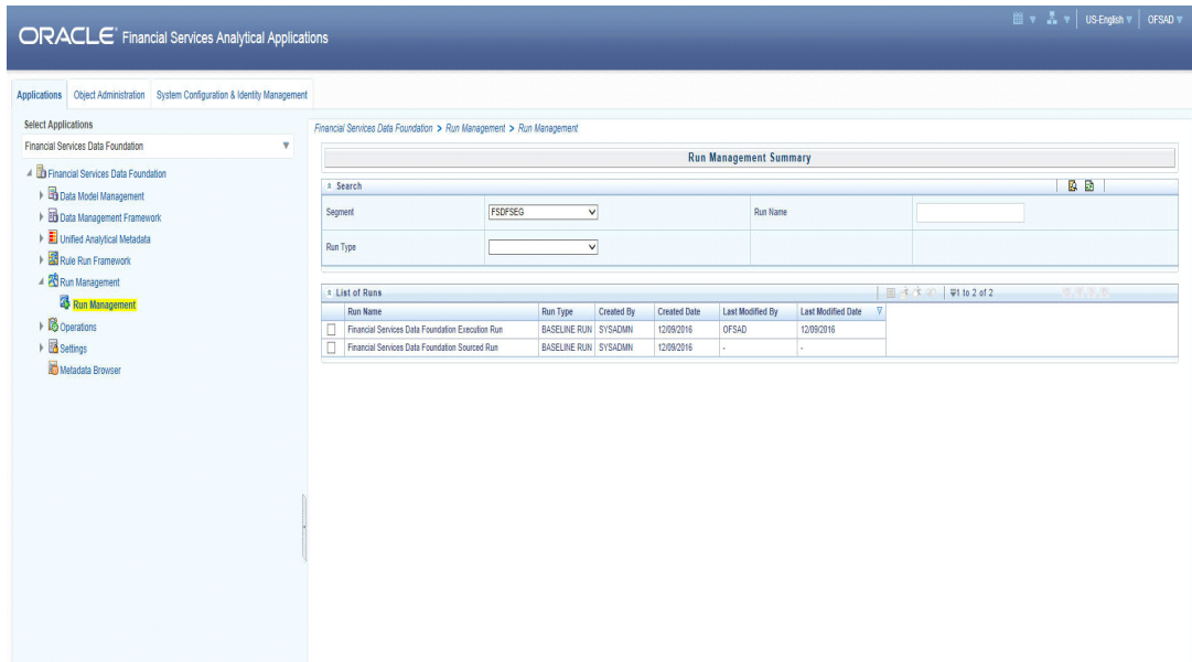
Figure 7. Search
